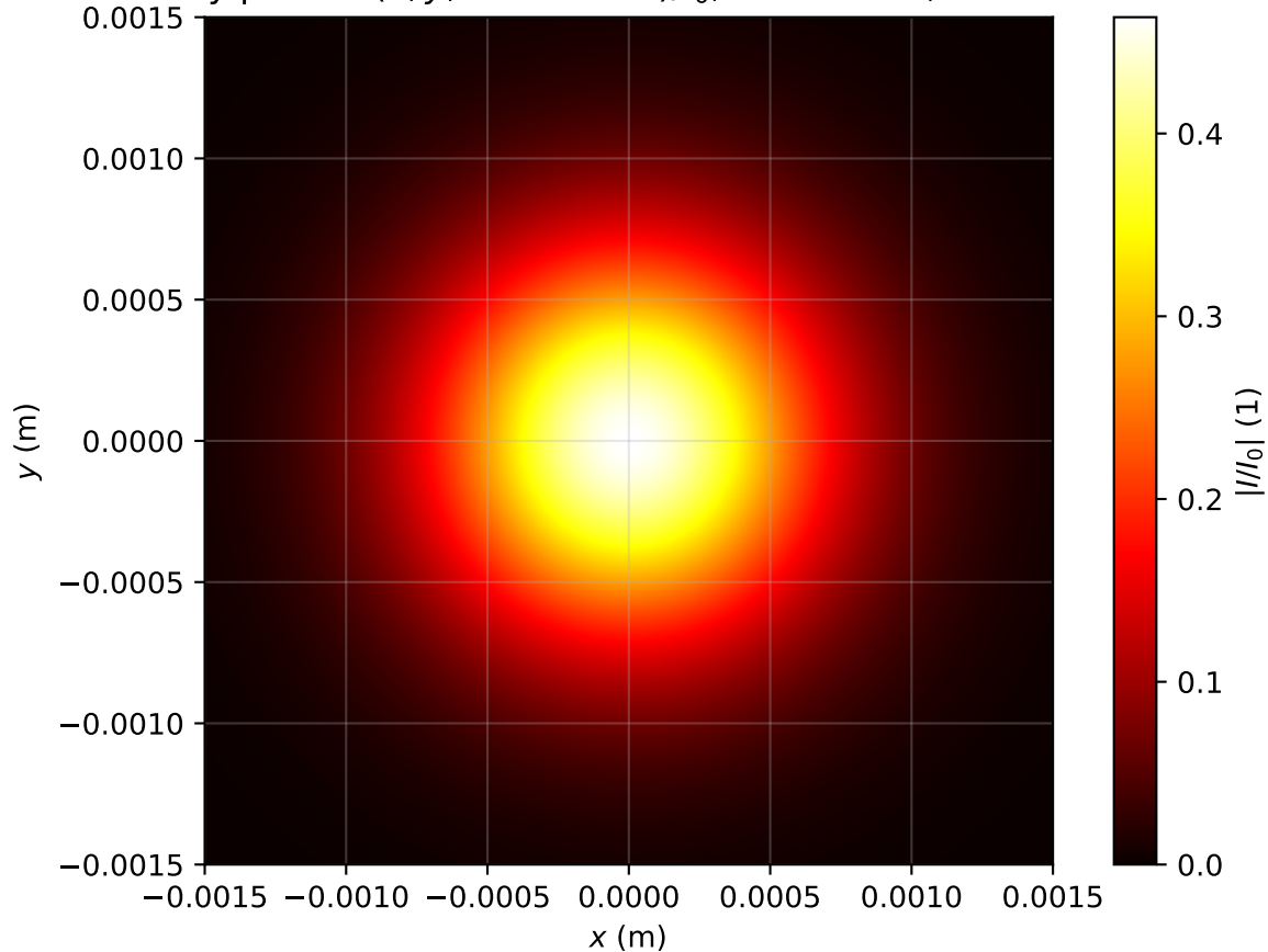
Intensity profile I(x, y, z = 2.786m)/I_0 , Pin=0.3Pcr, artificial time
